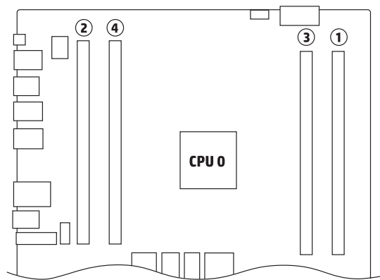
Figure 5. Loading order
